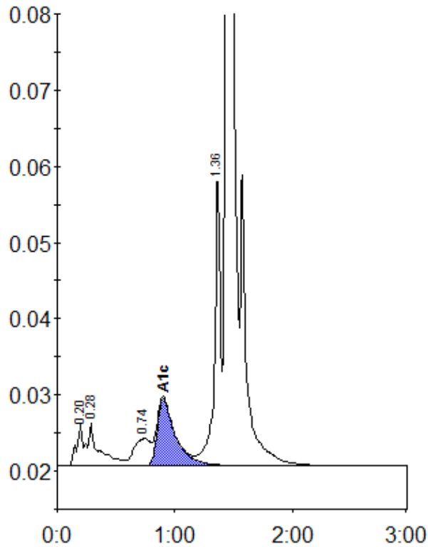
Peak table - ID: 10396341
